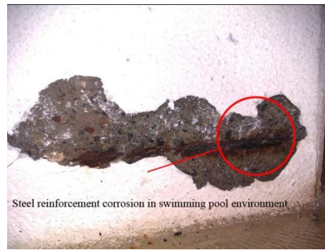
Figure5-Steel oxidization, Photo by author
