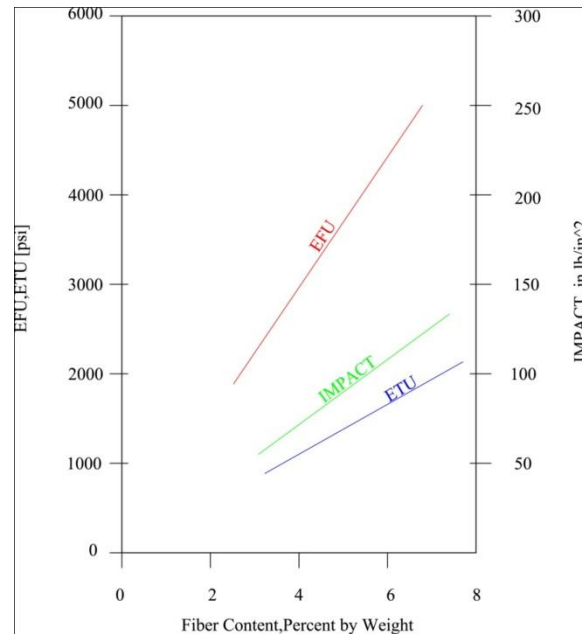
Figure 14 -Effect of fiber content on early tensile ultimate strength (ETU), [2]
