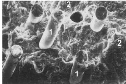
Figure 13-Glass fibers in matrix, [2]
