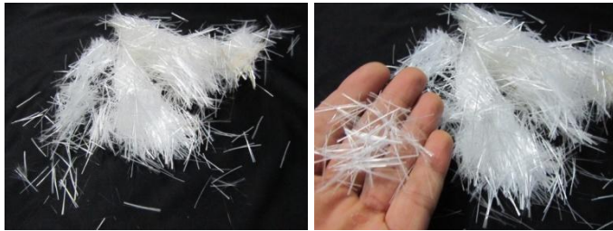
Figure6-GFRC chopped strands. 24 mm. Photo by author
