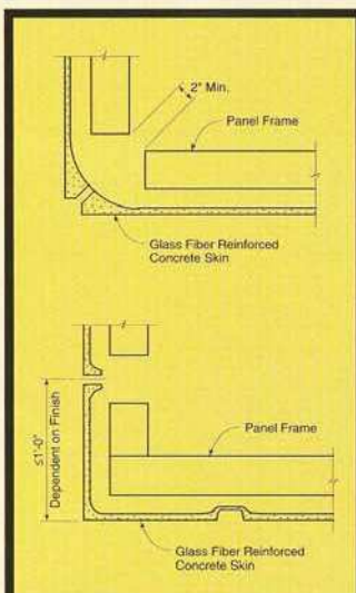
Panel Corner Details
