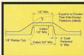
Reveal or False Joint
